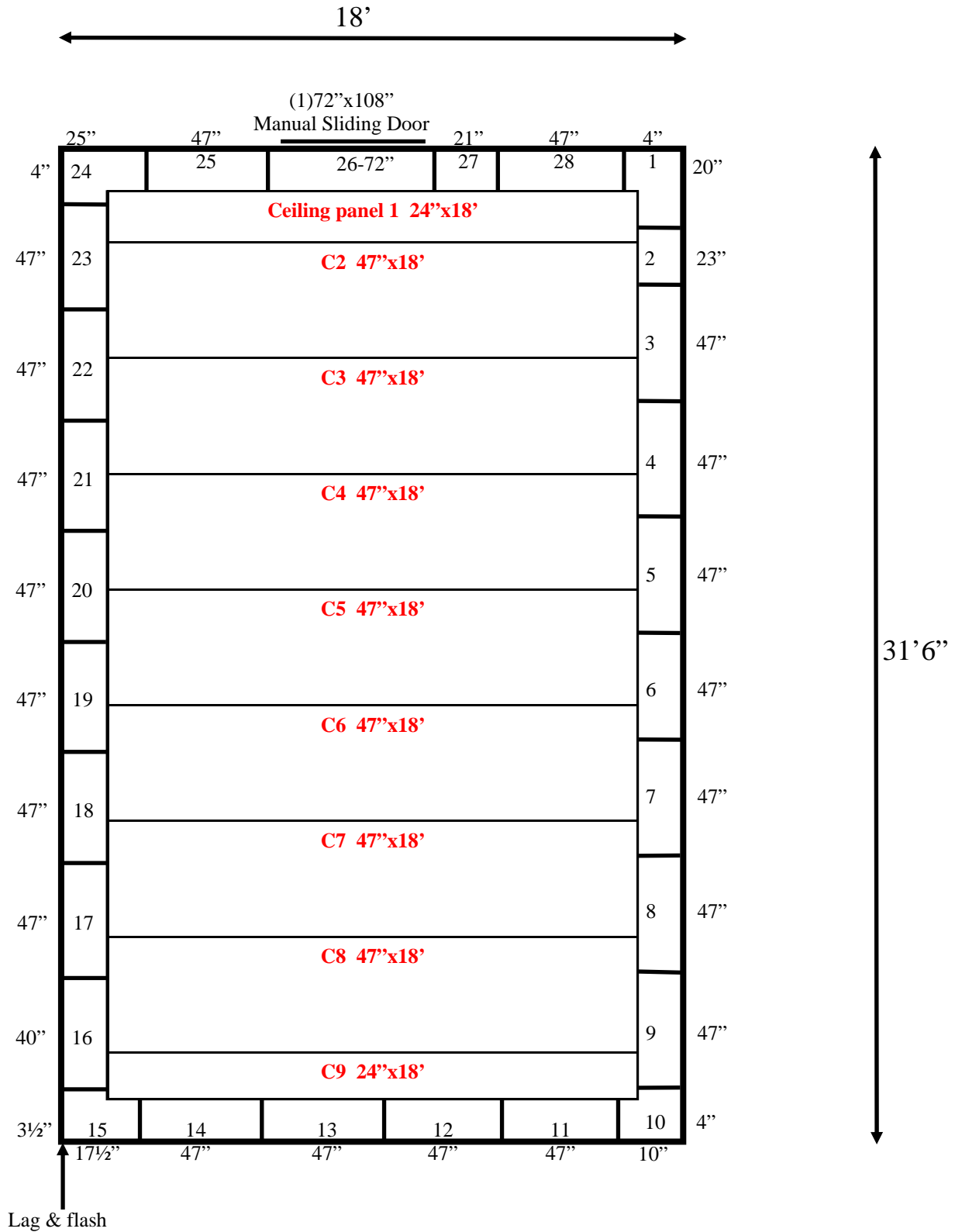
18' x 31'6" x 12' H Cooler Wall & Ceiling Panels Diagram
