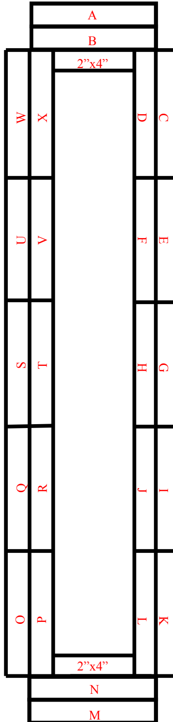
19' x 48' x 15'H and 16'H Cooler or Freezer Riser Diagram
