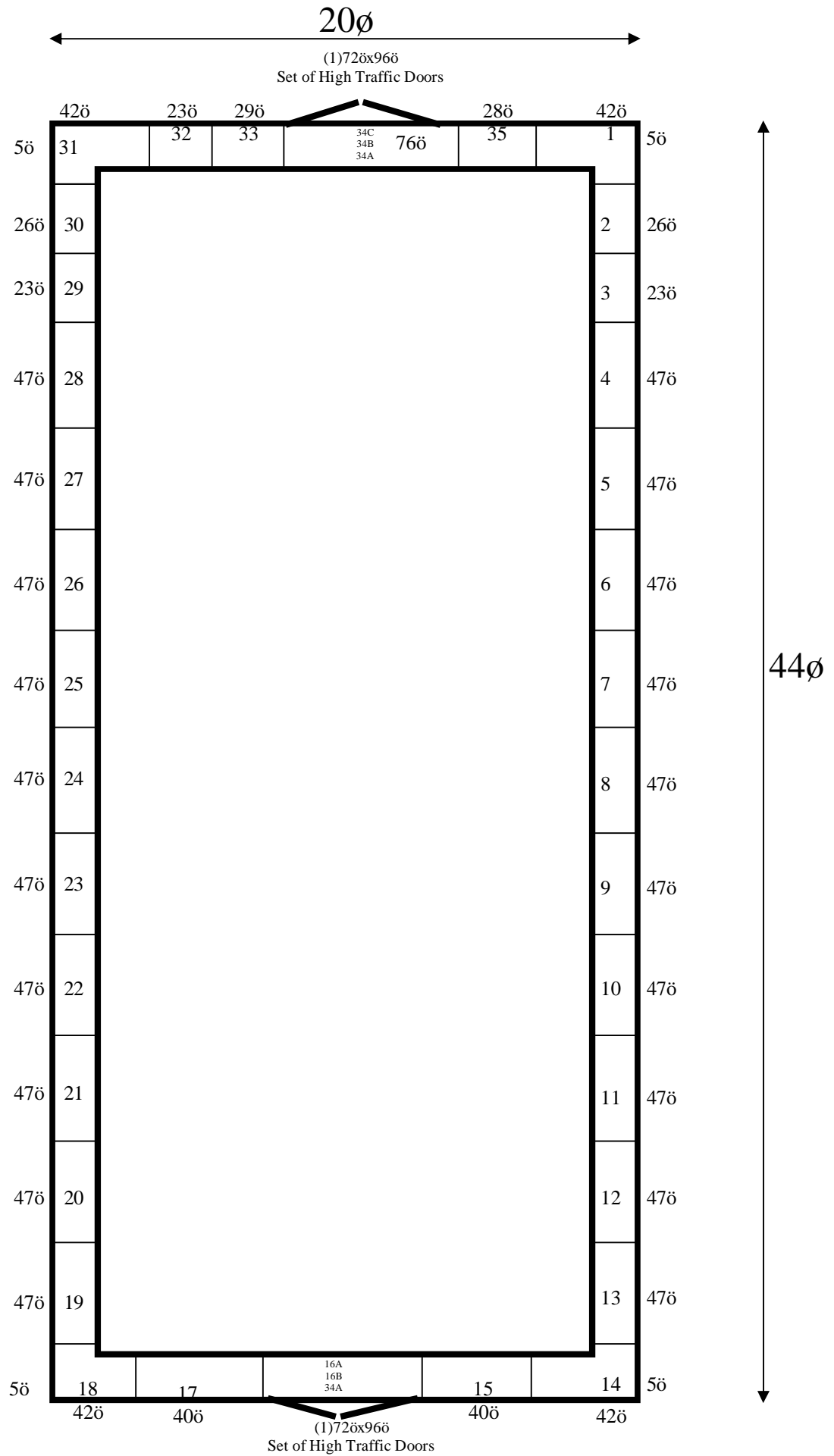
20' x 44' x 15' H and 16' H Cooler or Freezer Wall Panels Diagram
