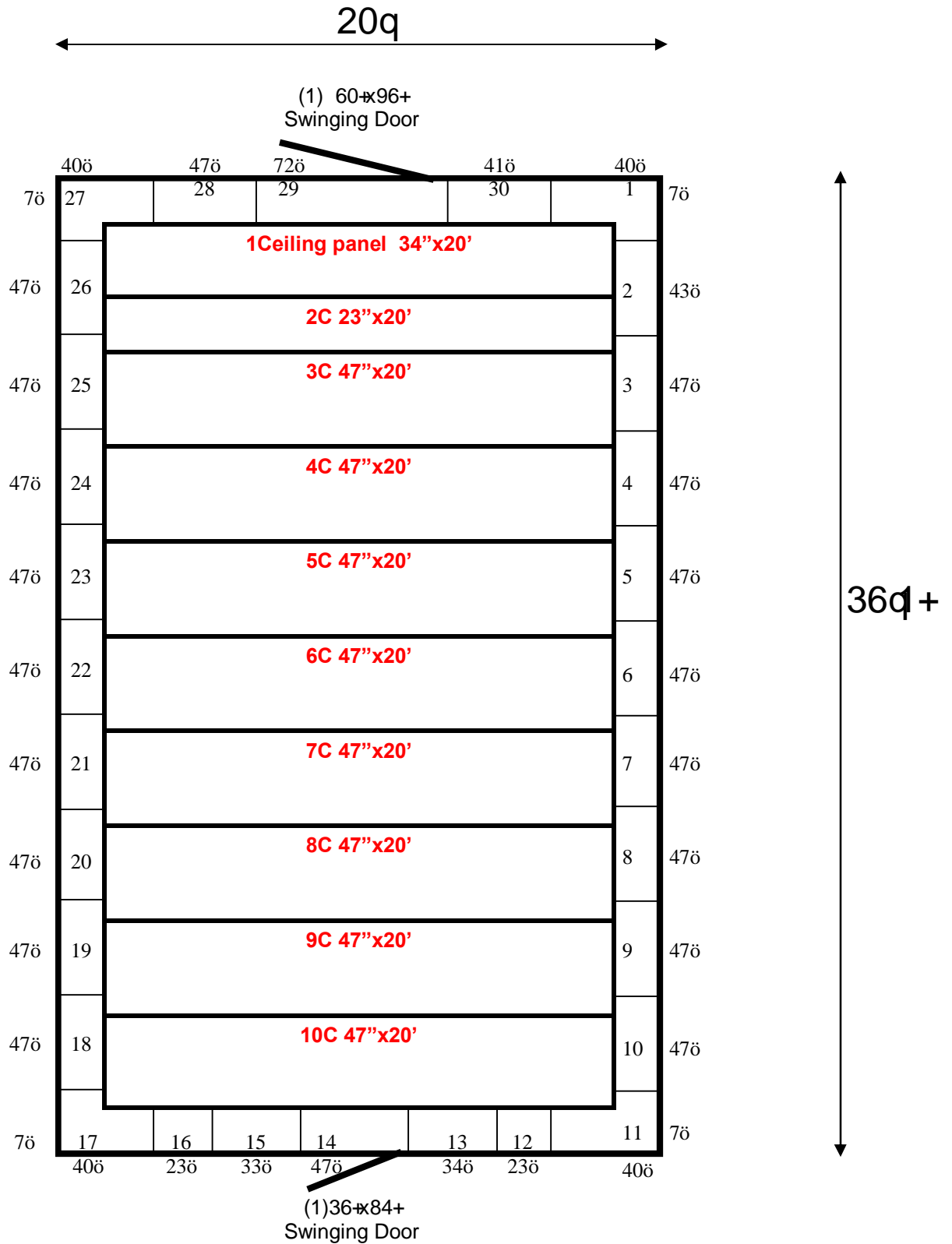
20' x 36'1" x 14' H Cooler or Freezer Wall & Ceiling Panels Diagram
