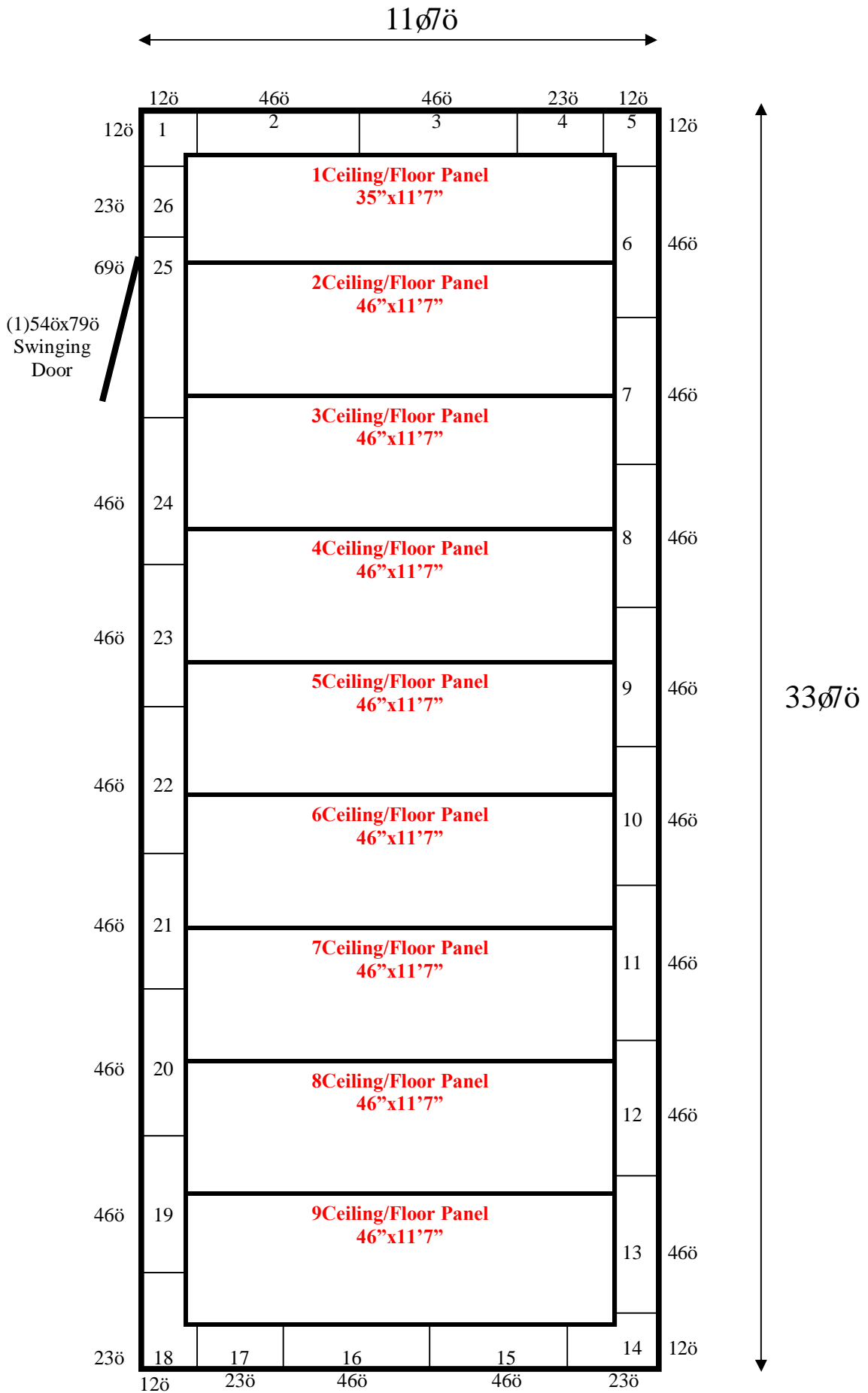
11'7" x 33'7" x 8'8" H Freezer With Floor Wall, Ceiling & Floor Panels Diagram
