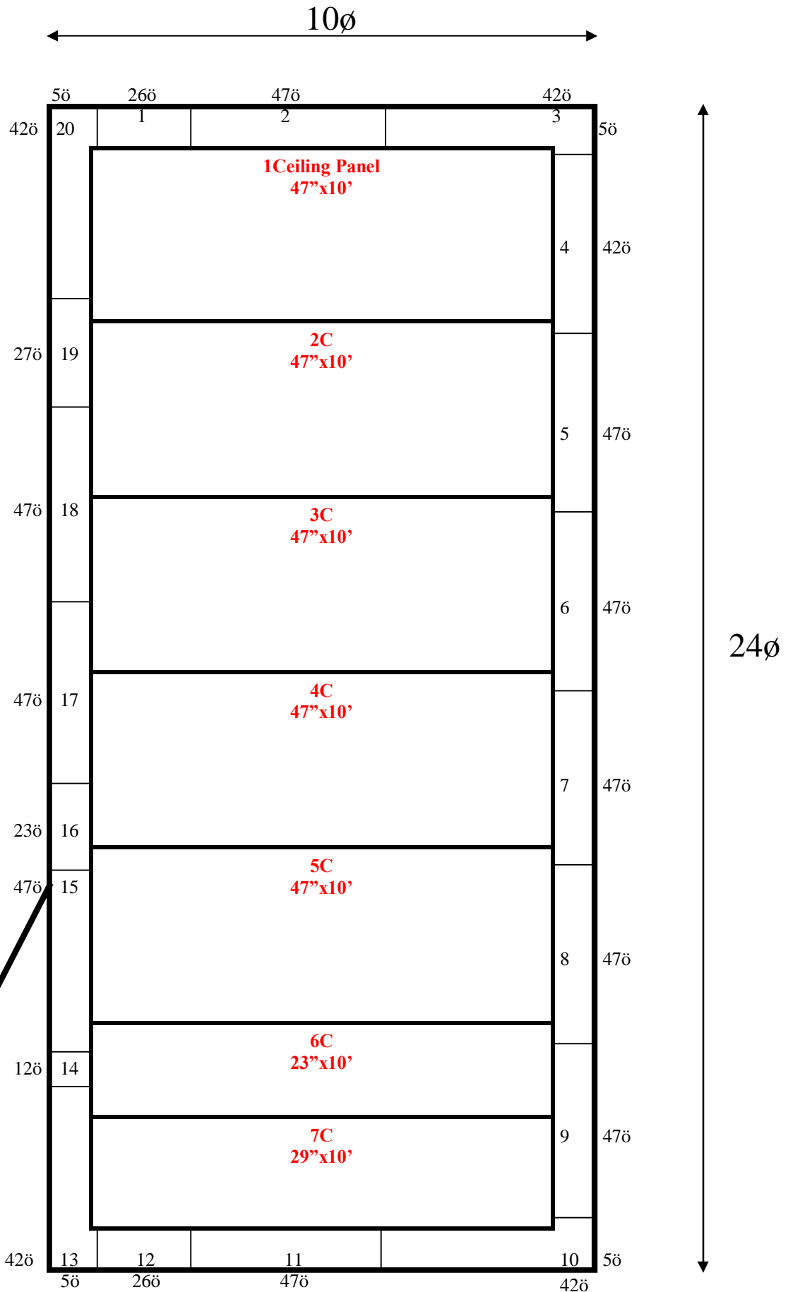
10' x 24' x 9'11" H Cooler Wall & Ceiling Panels Diagram
