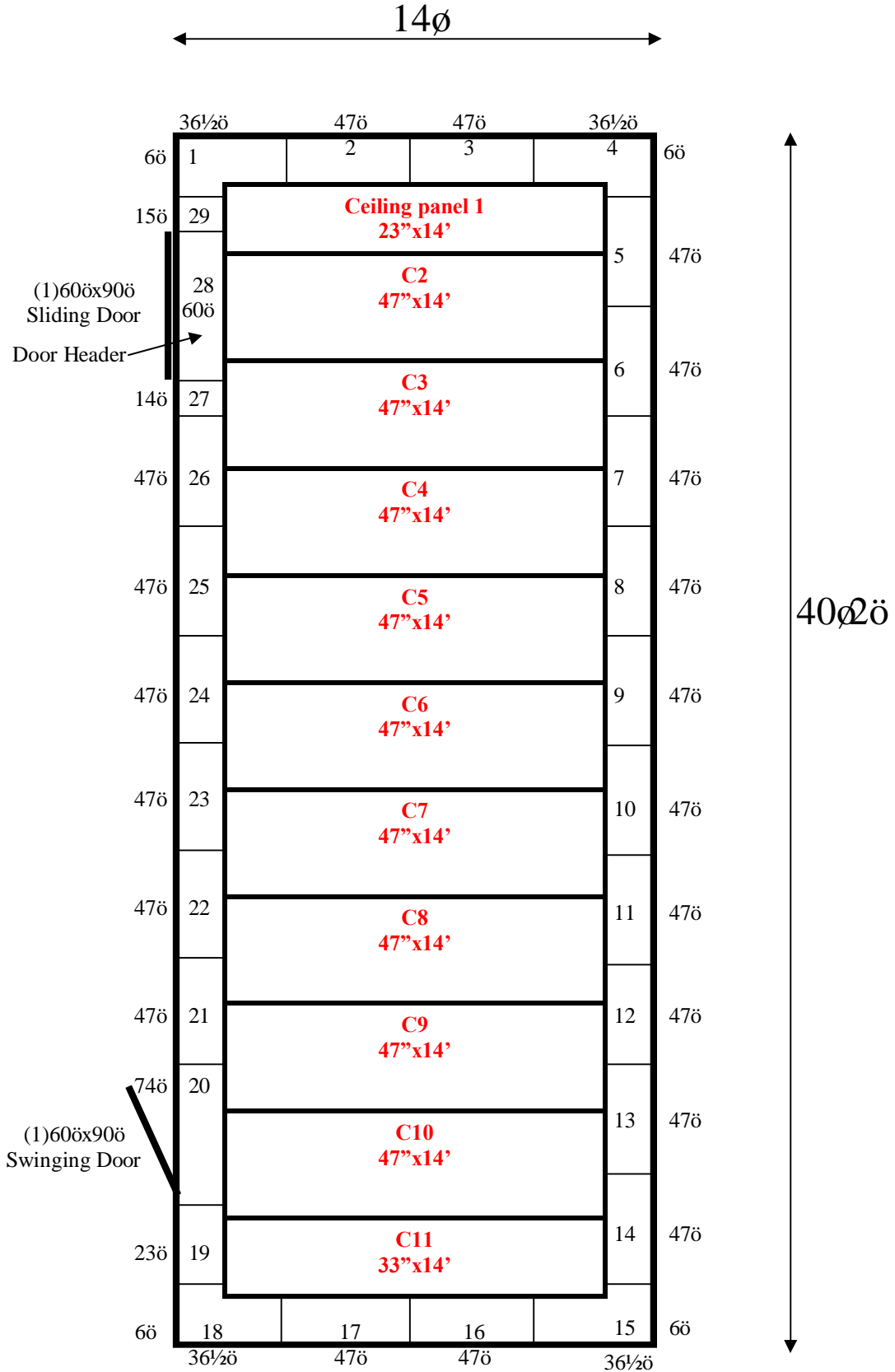
14' x 40'2" x 10' H Cooler or Freezer Wall & Ceiling Panels Diagram
