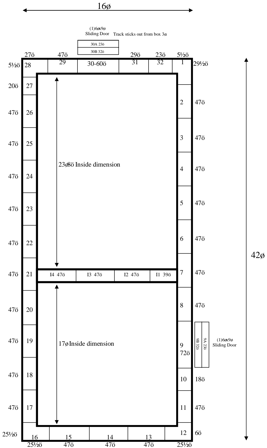
16' x 42' x 14' H Cooler or Freezer Wall Panels Diagram
