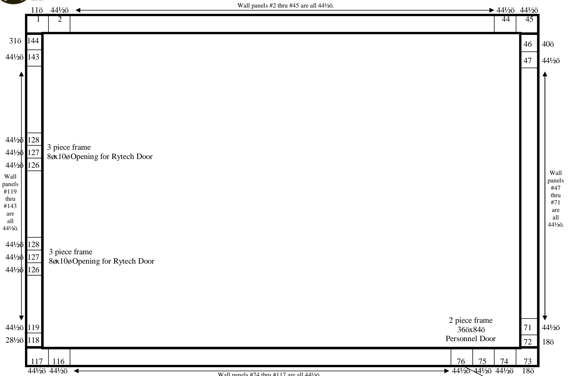
98'7" x 164' x 21'4" H Drive-In Cooler or Freezer Wall Panels Diagram
