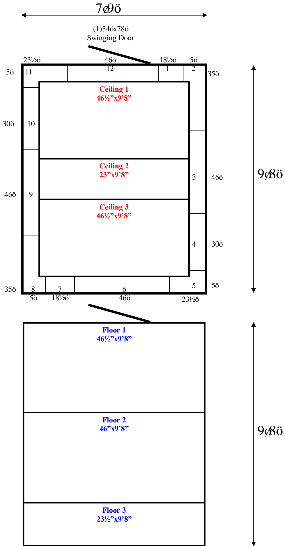
7'9" x 9'8" x 7'7" H Freezer with Floor Wall, Ceiling & Floor Panels Diagram
