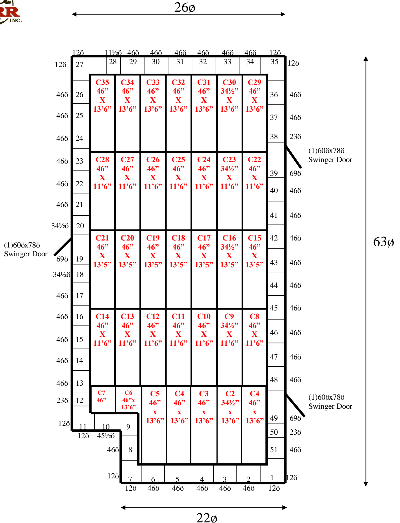
26' x 63' x 10' H Cooler Wall & Ceiling Panels Diagram
