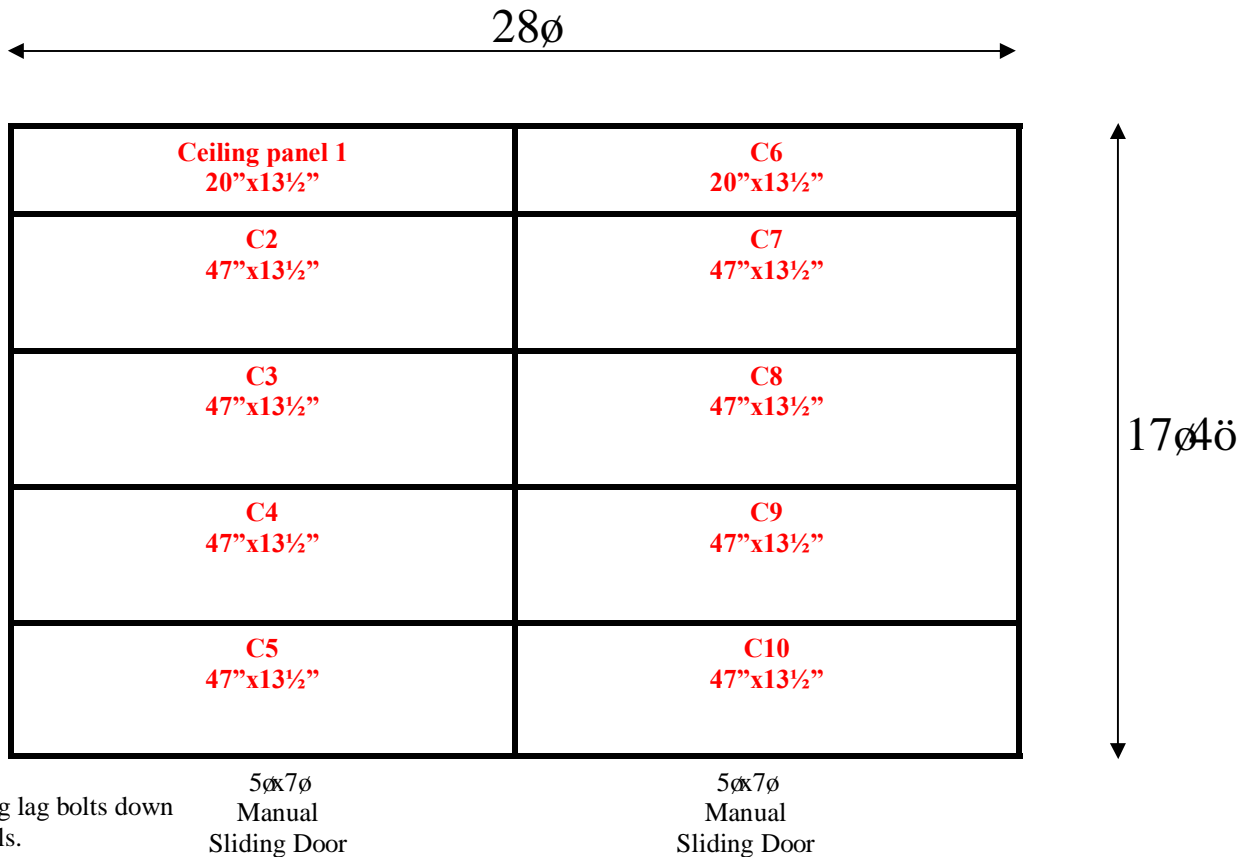
17'4" x 28' x 10'2" H Combination Walk-In Cooler / Freezer Wall & Ceiling Panels Diagram
