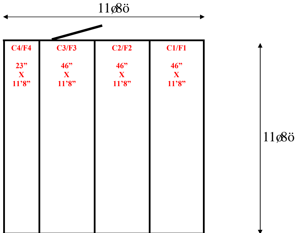
11'8" x 11'8" x 8'6" H Walk-In Freezer With Floor Wall, Ceiling & Floor Panels Diagram
