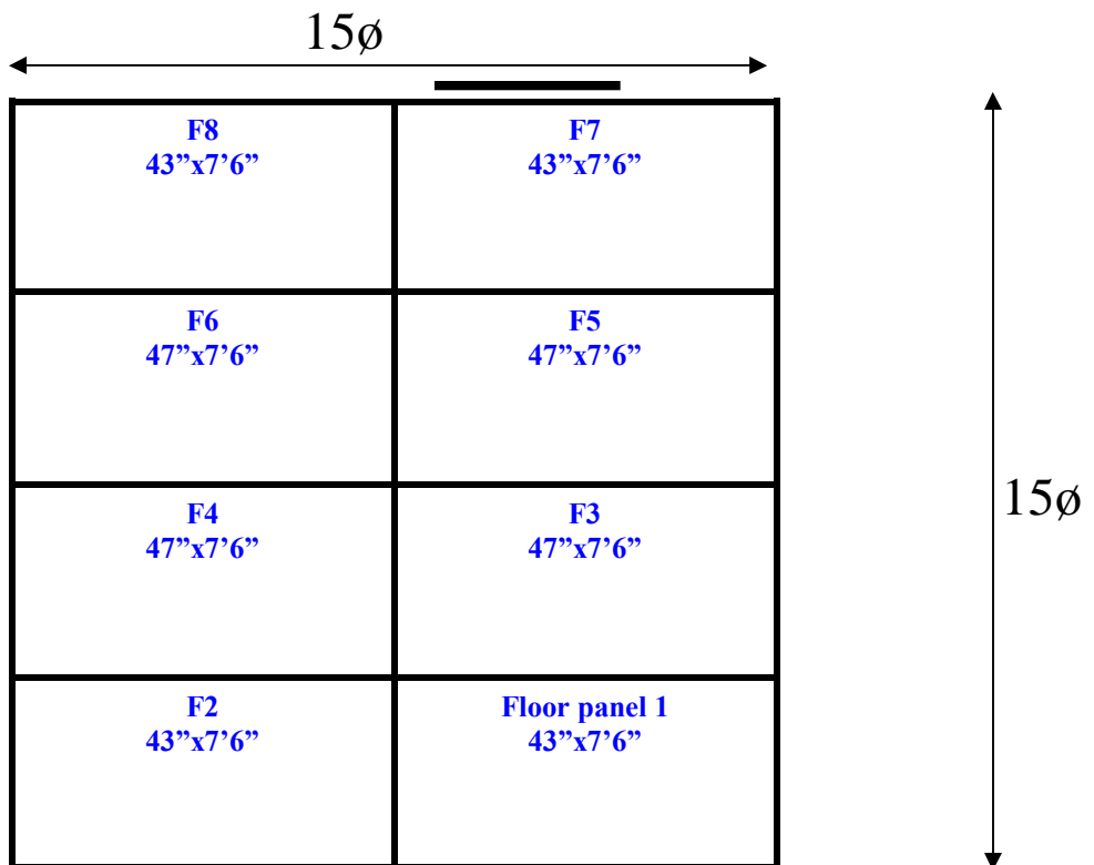
15' x 15' x 9'4" H Walk-In Freezer With Floor Wall, Ceiling & Floor Panel Diagrams
