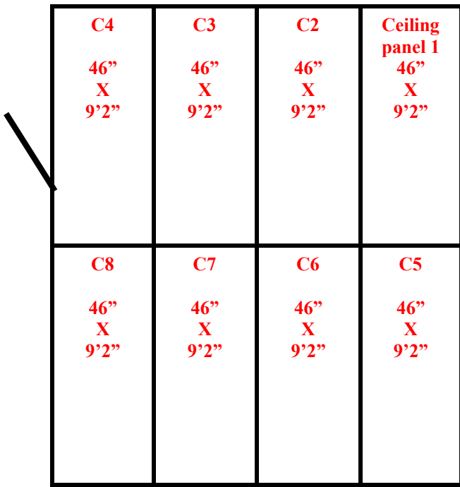
15'5" x 18'4" x 7'6" H Walk-In Combination Cooler / Freezer Wall, Ceiling & Floor Panel Diagrams
