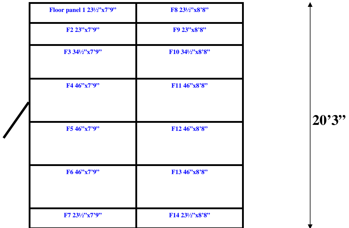
16'5" x 20'3" x 8'6" H Walk-In Freezer With Floor Wall, Ceiling & Floor Panel Diagrams
