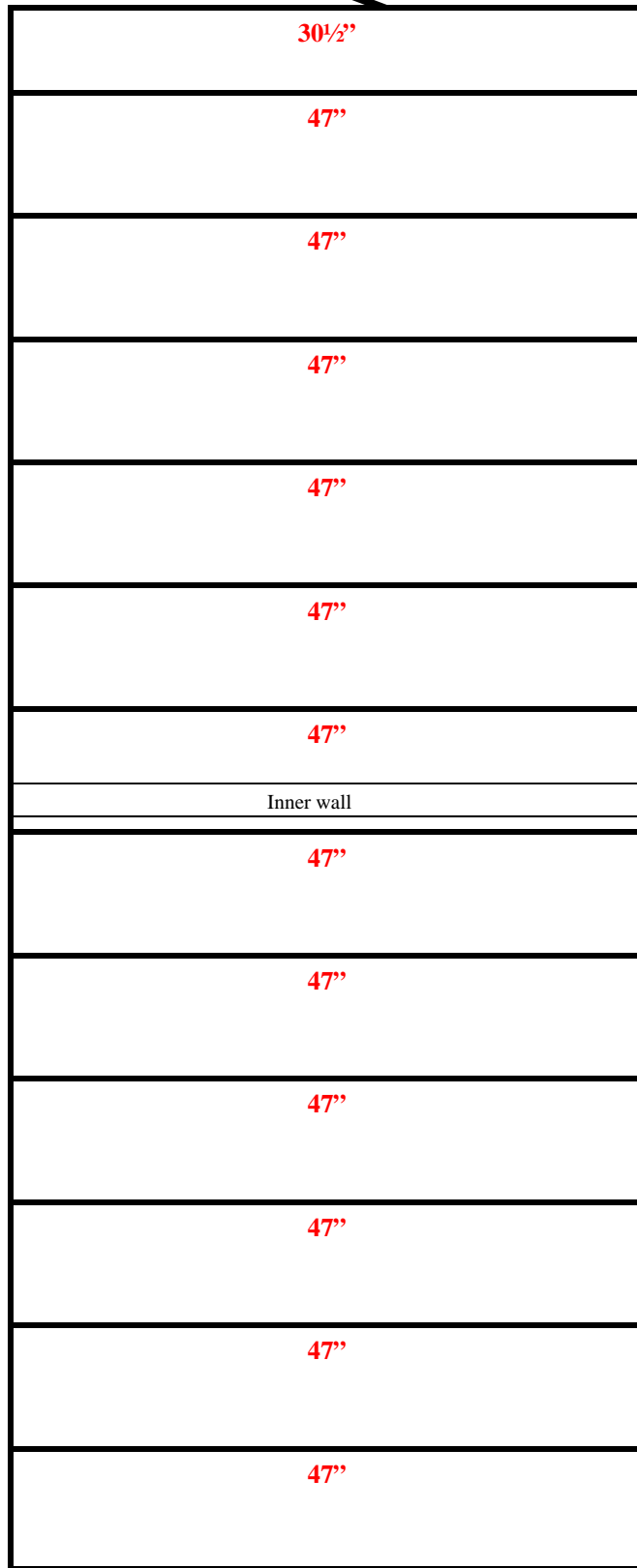
18' x 49'7" x 14' H Drive-In Cooler or Freezer Ceiling Panels Diagram
