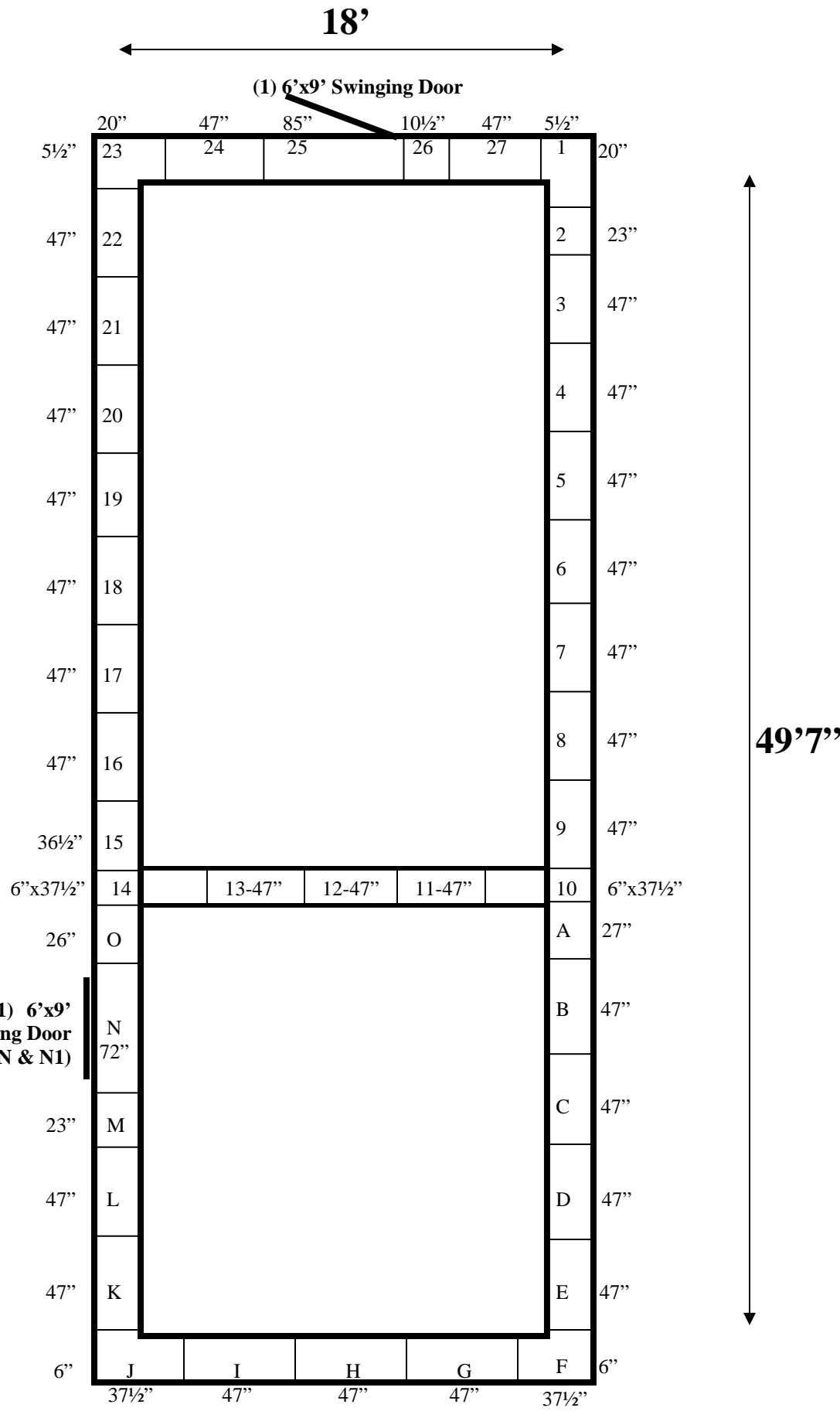
18' x 49'7" x 14' H Drive-In Cooler or Freezer Wall Panels Diagram
