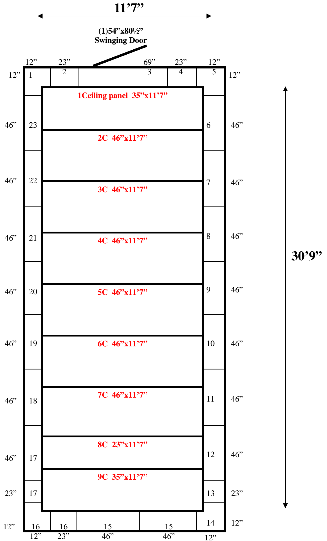
11'7" x 30'9" x 8'5" H Walk-In Cooler or Freezer Wall & Ceiling Panels Diagram
