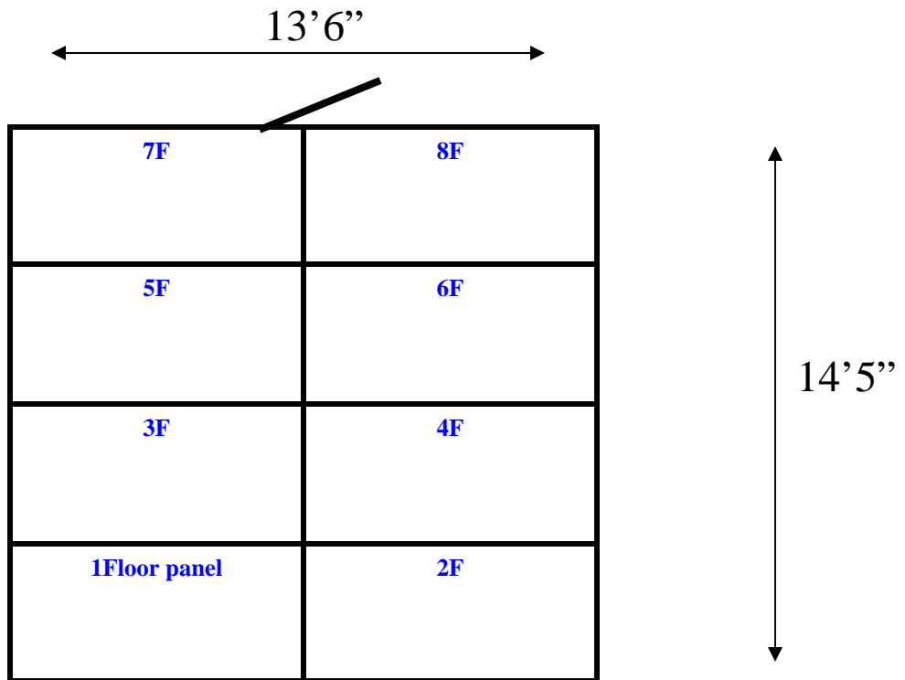
13'6" x 14'5" x 8'8" H Walk-In Freezer with Floor Wall, Ceiling & Floor Panels Diagrams
