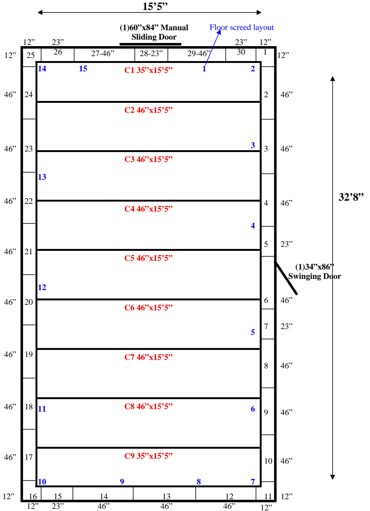
15'5" x 32'8" x 10'5" H Drive-In Cooler Wall & Ceiling Panels Diagram
