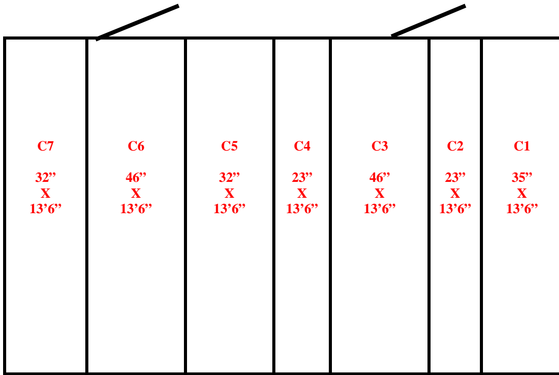
13'6" x 19' x 10'5" H Walk-In Combination Cooler/Freezer Wall & Ceiling Panels Diagram
