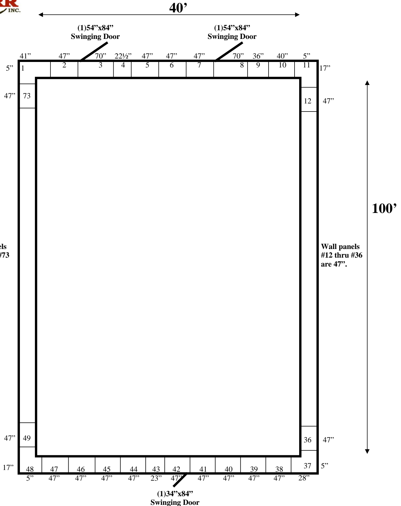
40' x 100' x 8' H Drive-In Cooler or Freezer Wall Panels Diagram
