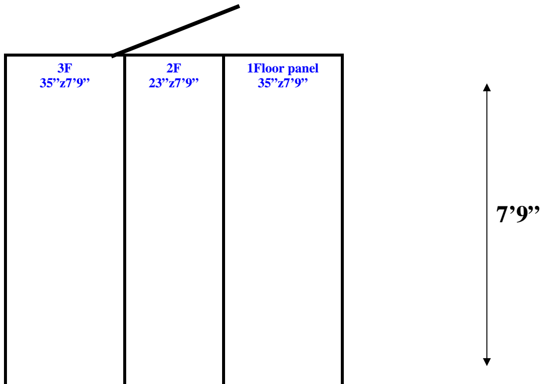
7'9" x 7'9" x 8'8" H Walk-In Freezer With Floor Wall, Ceiling & Floor Panels Diagram
