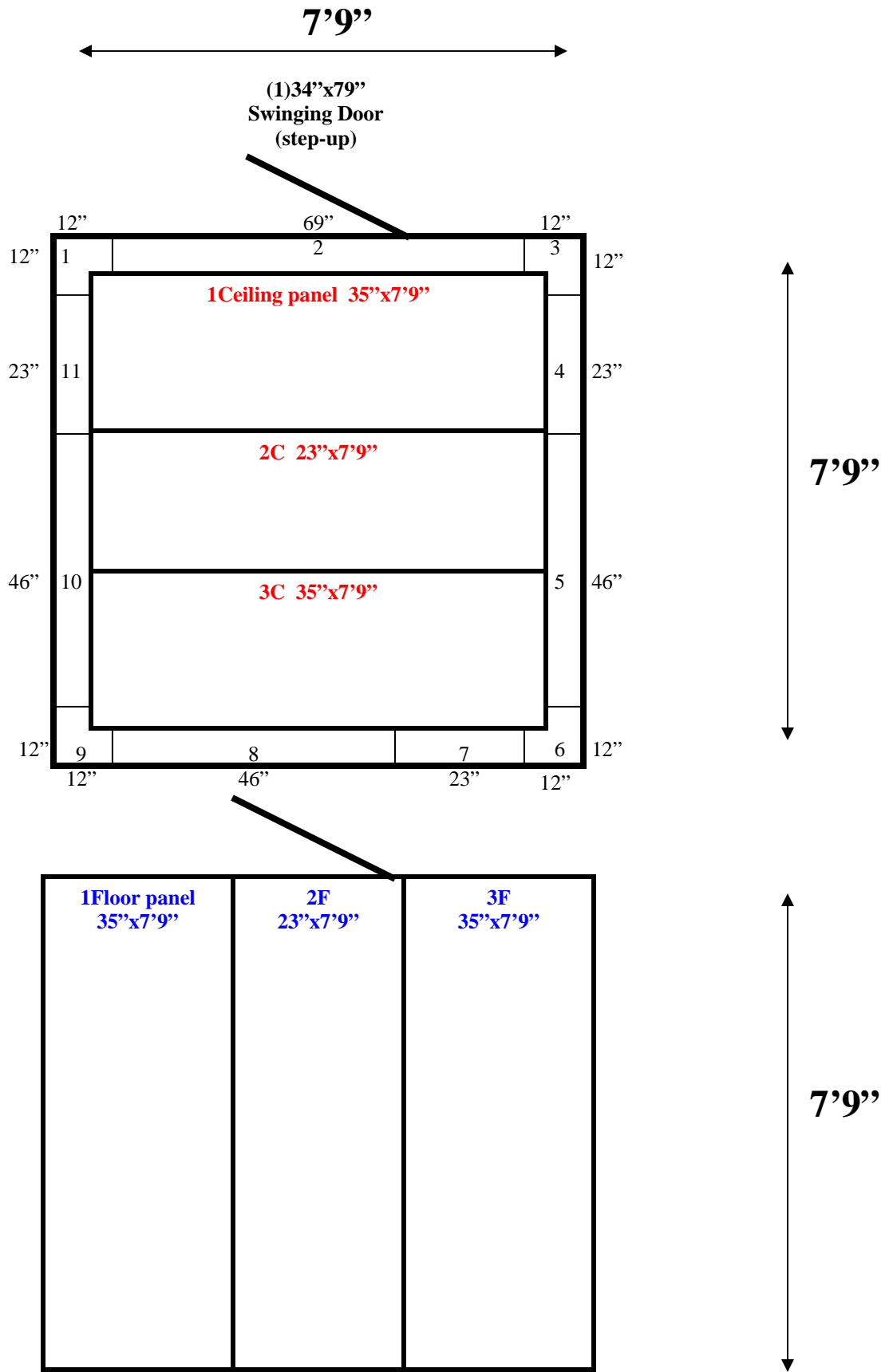
7'9" x 7'9" x 8'8" H Walk-In Freezer With Floor Wall, Ceiling & Floor Panels Diagram
