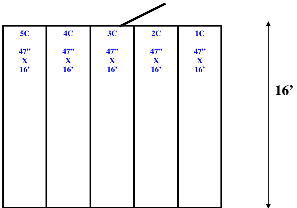
16' x 17' x 9'6" H Walk-In Freezer With Floor Wall, Ceiling & Floor Panel Diagrams
