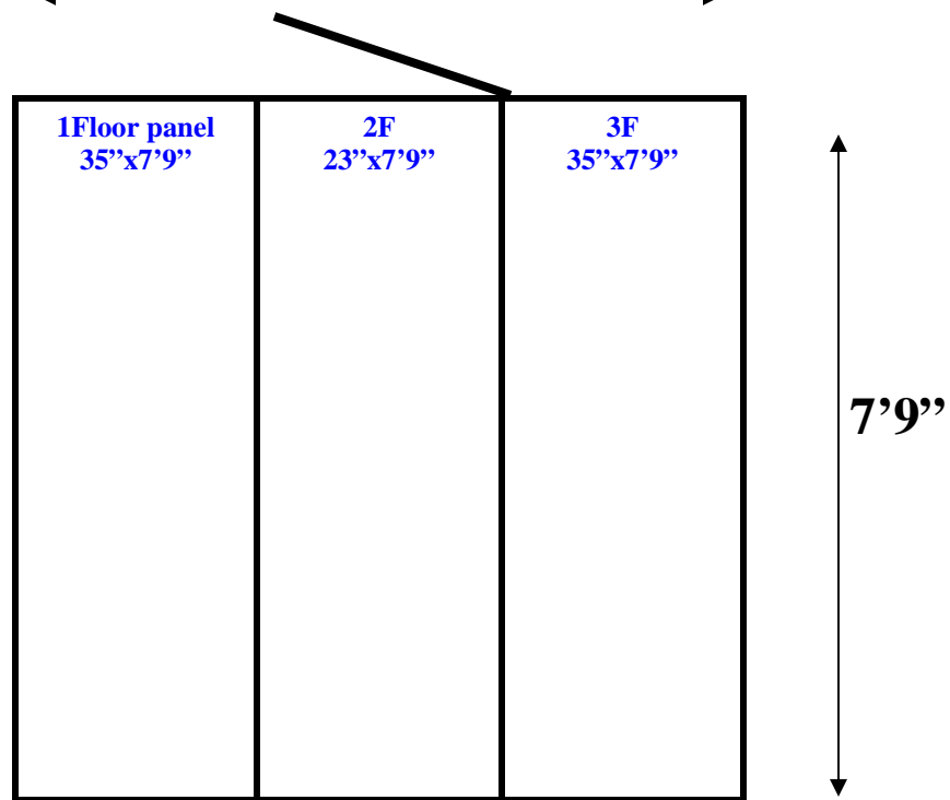
7'9" x 7'9" x 8'8" H Walk-In Freezer With Floor Wall, Ceiling & Floor Panels Diagram
