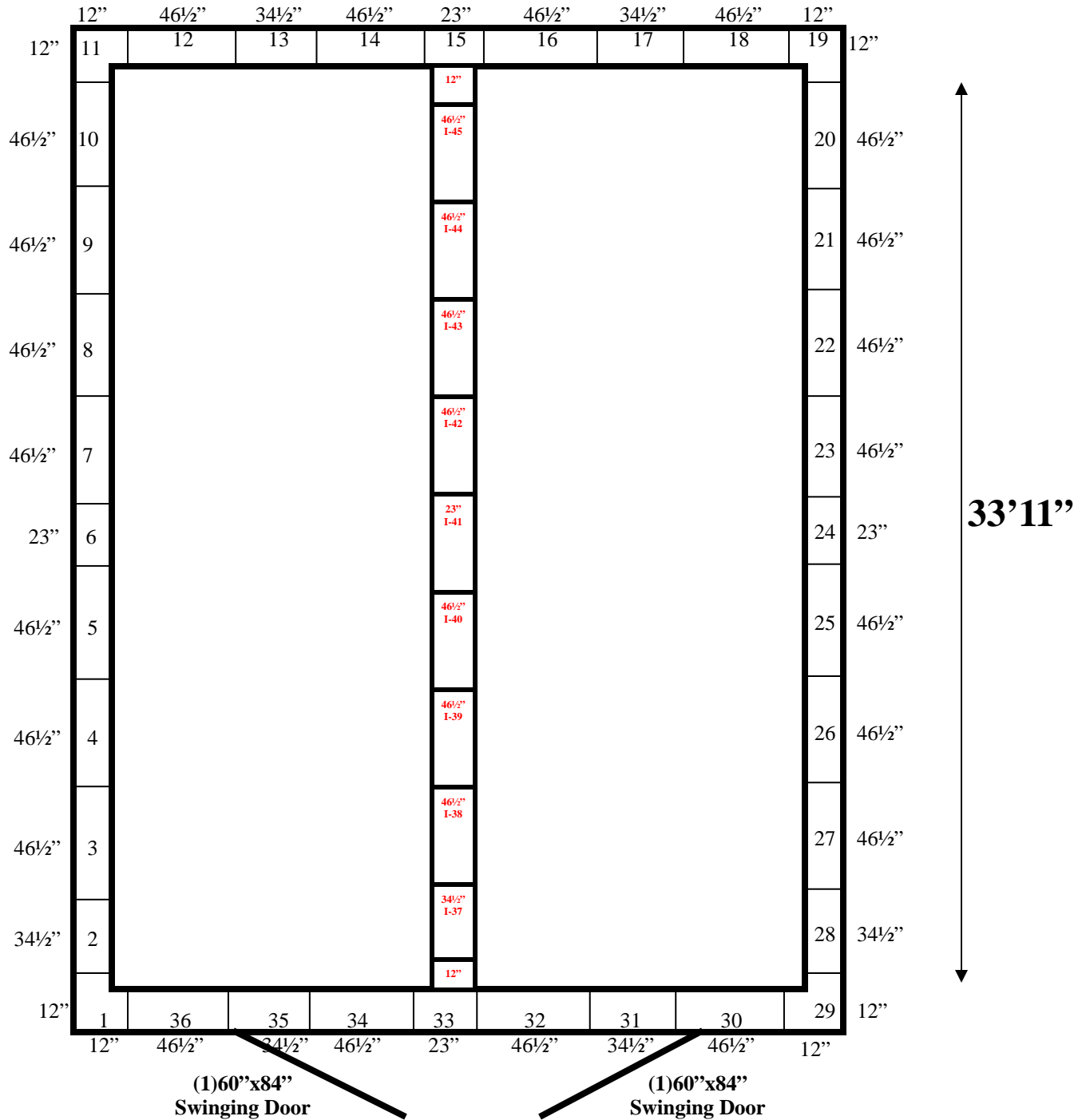
25'2" x 33'11" x 11'7" H Combination Walk-In Freezer With Floor Wall Panels Diagram
