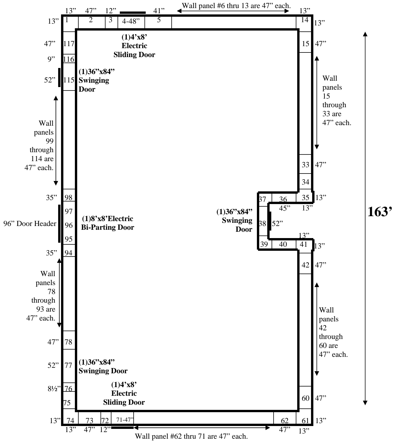
45'10" x 163' x 14' H Drive-In Cooler or Freezer Wall Panels Diagram
