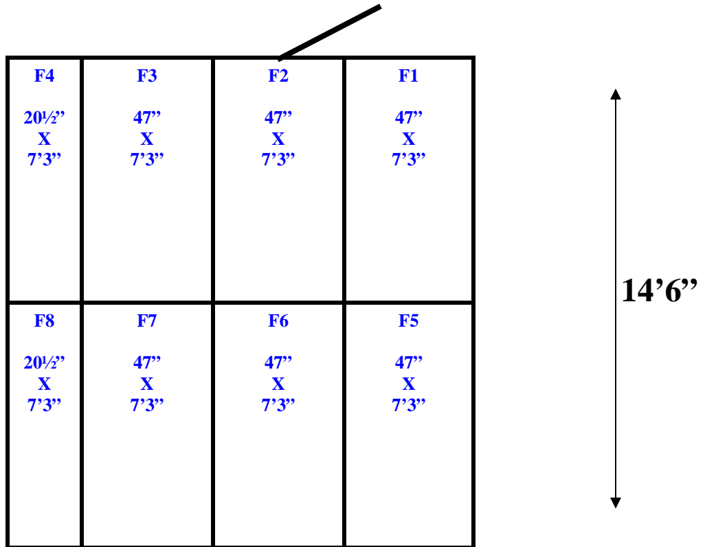
13'6" x 14'6" x 8'8" H Walk-In Freezer With Floor Wall, Ceiling & Floor Panels Diagram
