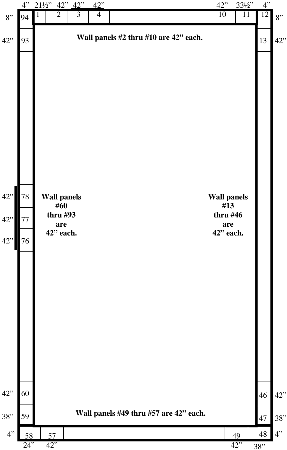
36'9" x 123'9" x 16'2" H Drive-In Cooler or Freezer Wall Panels Diagram
