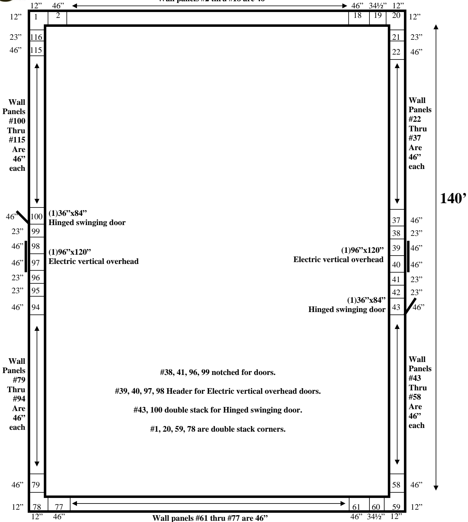
70' x 140' x 20' H Drive-In Cooler or Freezer Wall Panels Diagram
