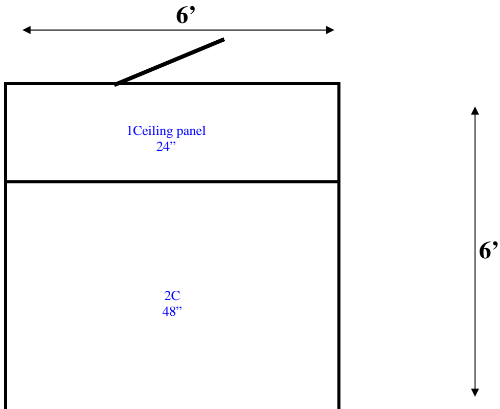
6' x 6' x 6'7" H (with unit 8' H) Walk-In Freezer With Floor Wall, Ceiling & Floor Panel Diagrams
