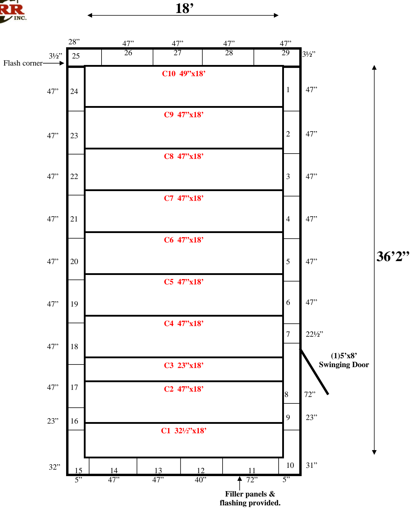
18' x 36'2" x 9'4" H Walk-In Cooler or Freezer Wall & Ceiling Panels Diagram
