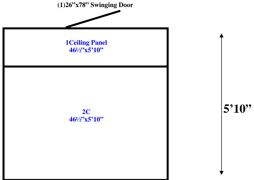
5'10" x 5'10" x 7'6" H (9'2" H with unit) Walk-In Cooler With Floor Wall, Ceiling & Floor Panels Diagram
