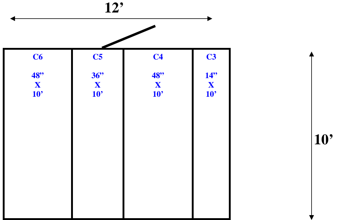
10' x 12'2" x 8'8" H Walk-In Freezer With Floor Wall, Ceiling & Floor Panels Diagram
