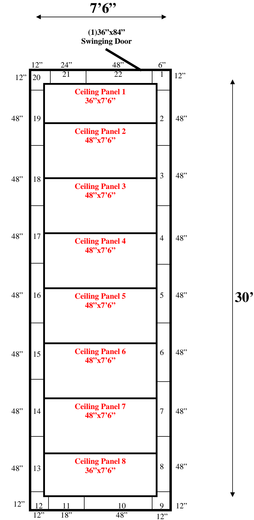
7'6" x 30' x 9'3" H Walk-In Cooler or Walk-In Freezer Wall & Ceiling Panels Diagram
