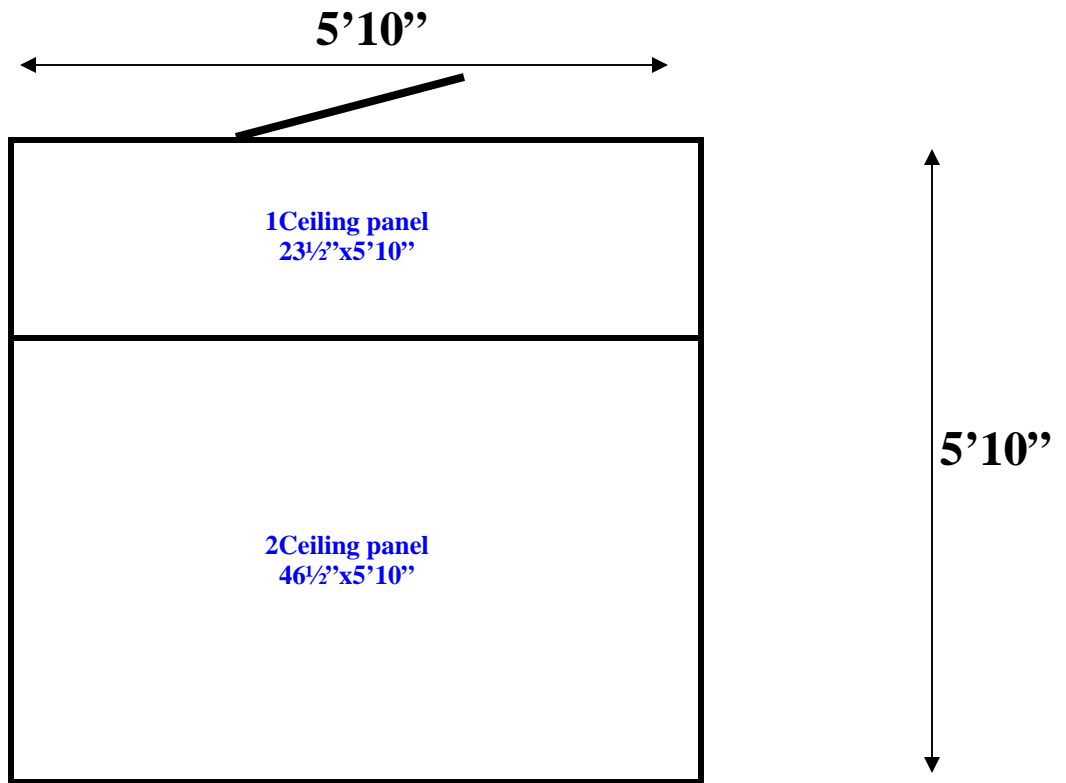
5'10" x 5'10" x 7'6" H (with unit 9'3" H) Walk-In Freezer with Floor Wall, Ceiling & Floor Panels Diagram
