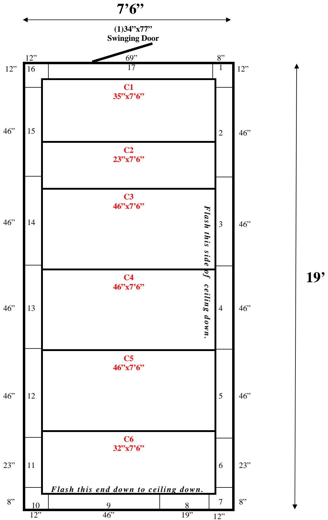
7'6" x 19' x 7'6" H Walk-In Cooler Wall & Ceiling Panels Diagram
