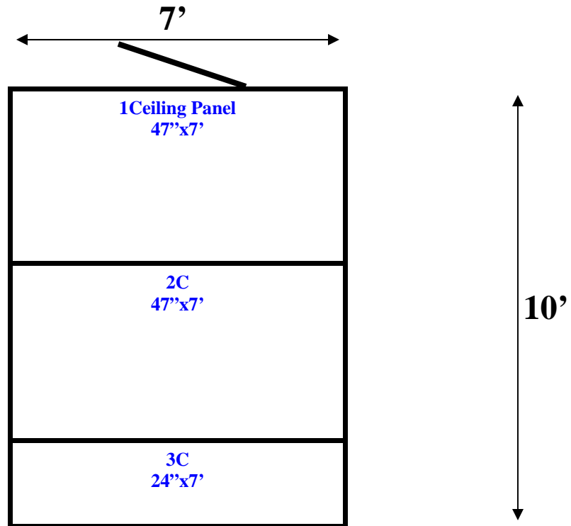
7' x 10' x 8' H Walk-In Freezer with Floor Wall, Floor & Ceiling Panel Diagrams
