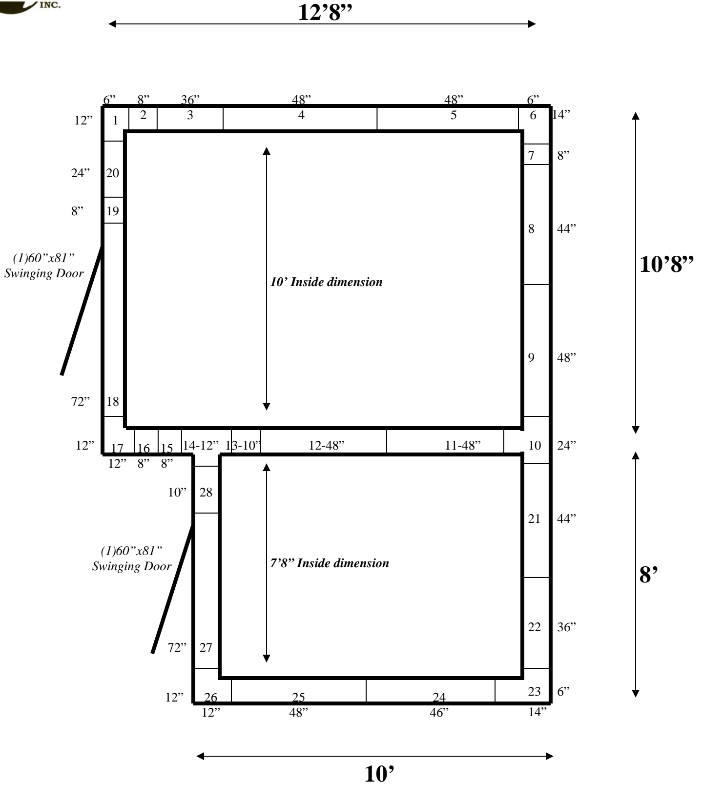
12'8" x 18'9" x 10'4" H Combination Walk-In Cooler/Walk-In Freezer Wall Panels Diagram
