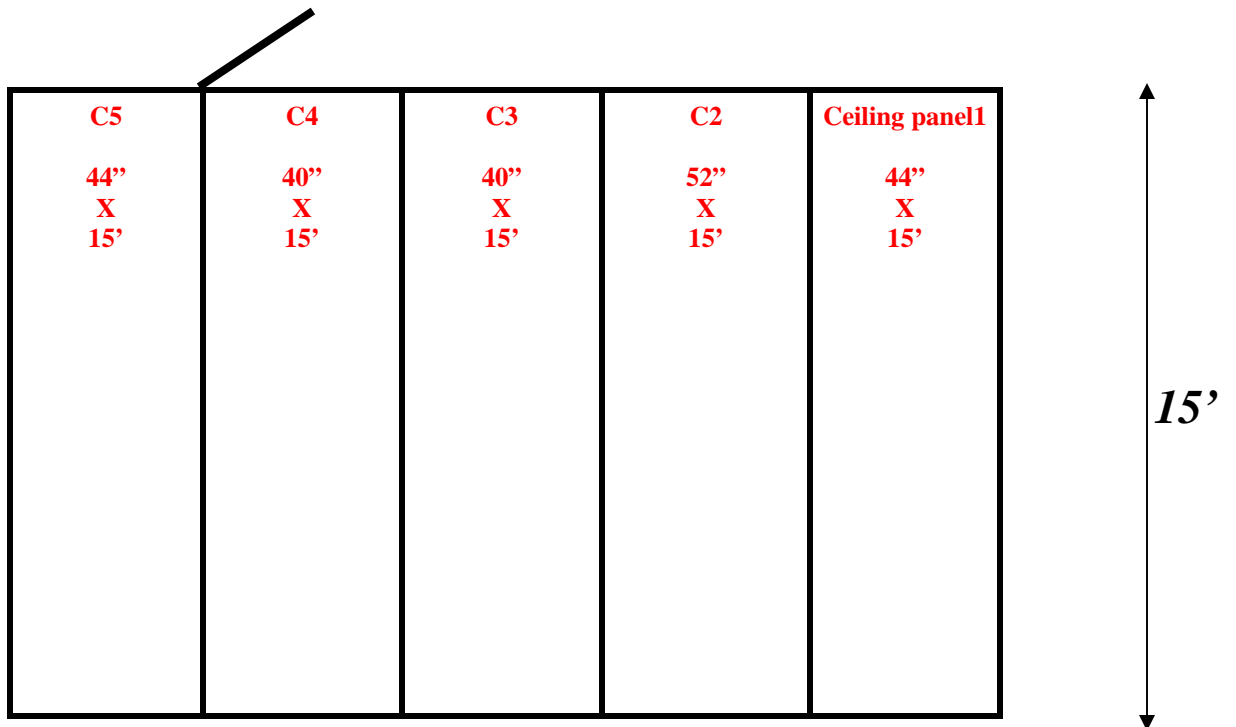
15' x 18'4" x 10' H Walk-In Cooler or Walk-In Freezer Wall & Ceiling Panels Diagram
