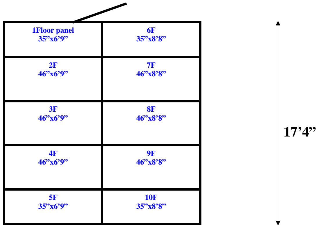
15'5" x 17'4" x 8'8" H Walk-In Freezer With Floor Wall, Ceiling & Floor Panels Diagram
