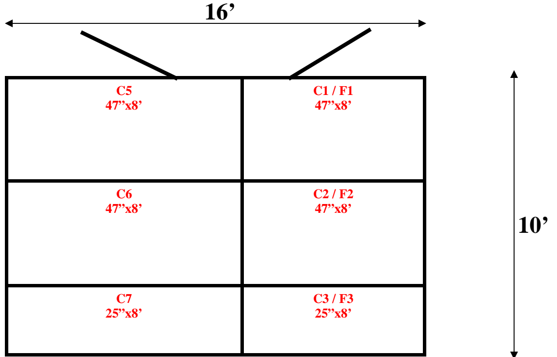
10' x 16' x 9' H Combination Walk-In Cooler/ Walk-In Freezer with Floor Wall, Ceiling & Floor Panels Diagram
