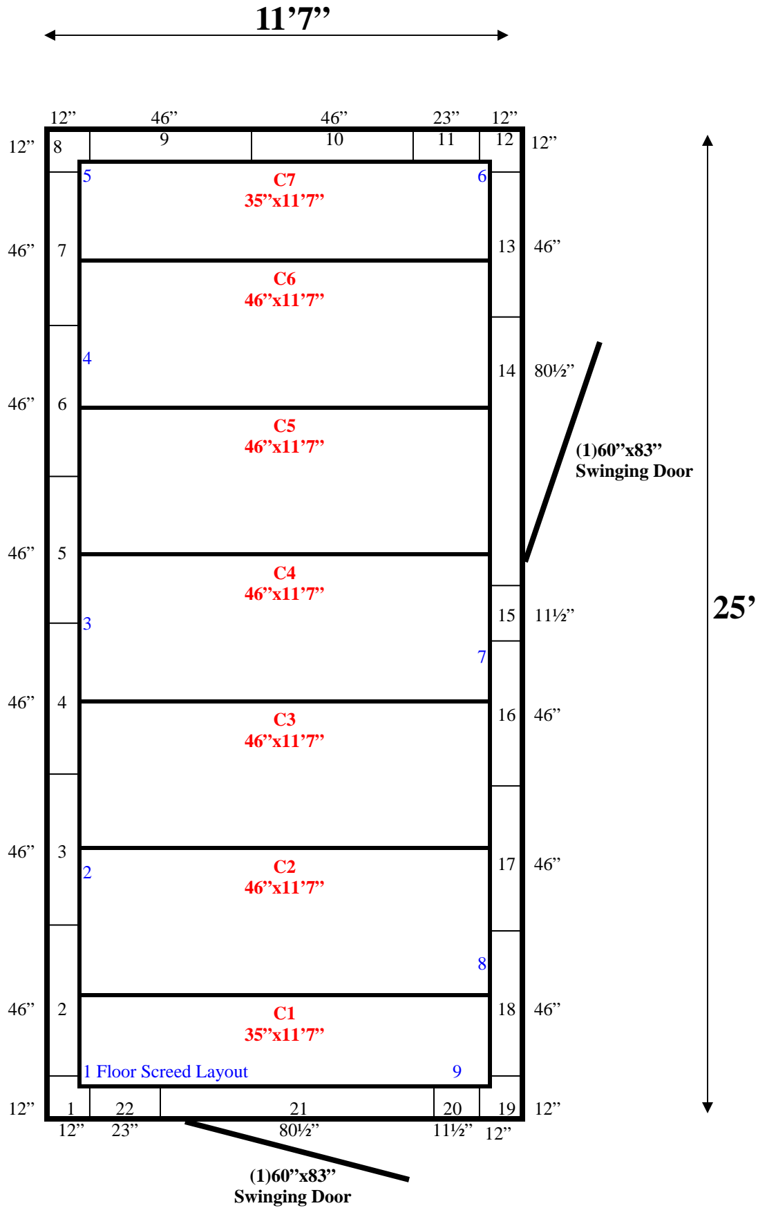
11'7" x 25' x 10'4" H Walk-In Cooler or Walk-In Freezer Wall & Ceiling Panels Diagram
