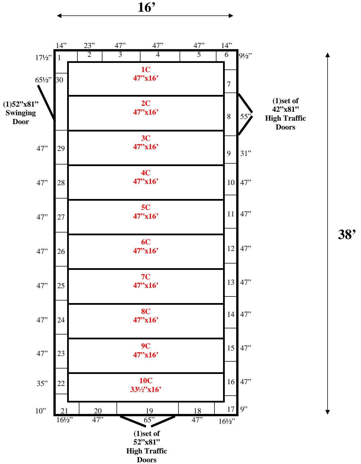
16' x 38' x 8'4" H Walk-In Cooler or Walk-In Freezer Wall & Ceiling Panels Diagram
