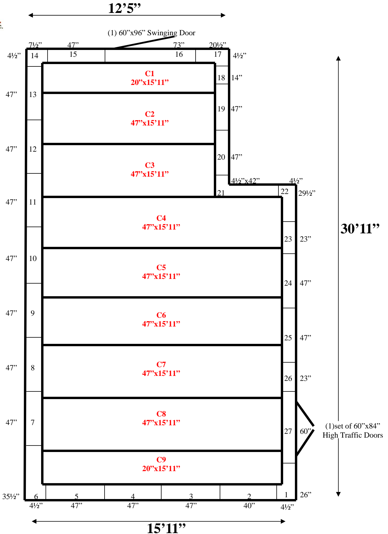
15'11" x 30'11" x 10' H Walk-In Cooler or Walk-In Freezer Wall & Ceiling Panels Diagram
