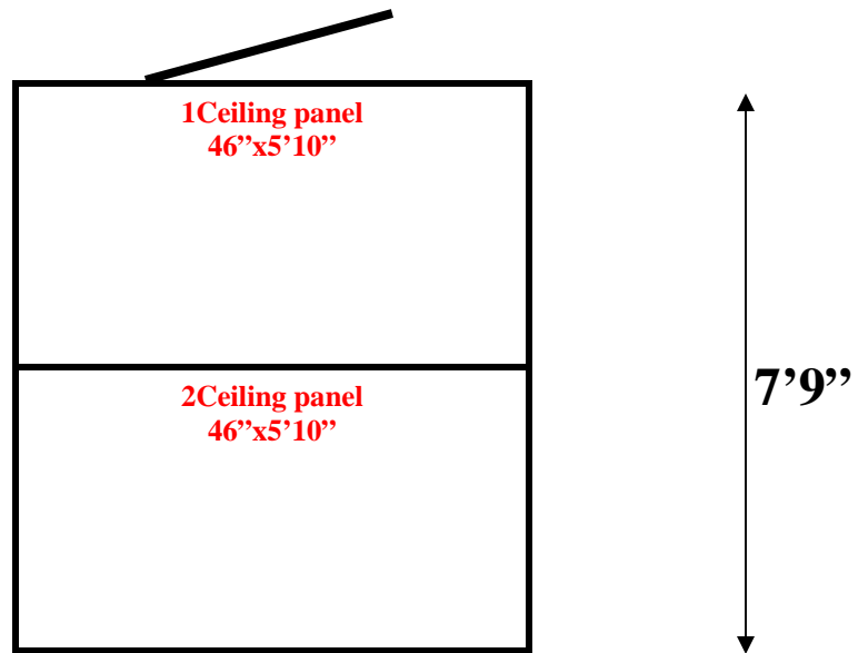
5'10" x 7'9" x 7'6" H (9'3"H with unit) Walk-In Freezer with Floor Wall, Floor & Ceiling Panel Diagrams
