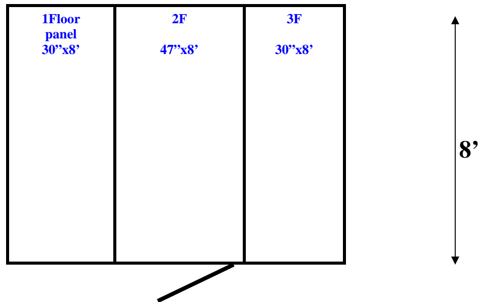
8' x 9' x 8'6" H Walk-In Freezer with Floor Wall, Ceiling & Floor Panel Diagrams
