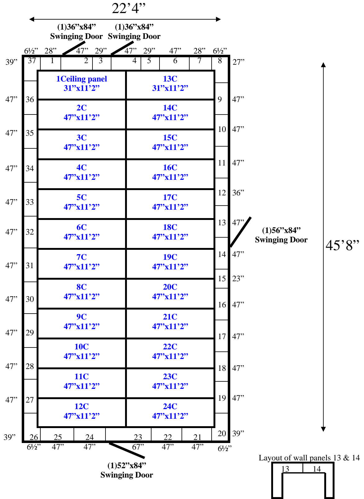
22'4" x 45'8" x 9'6" H Walk-In Freezer with Floor Wall & Ceiling Panels Diagram
