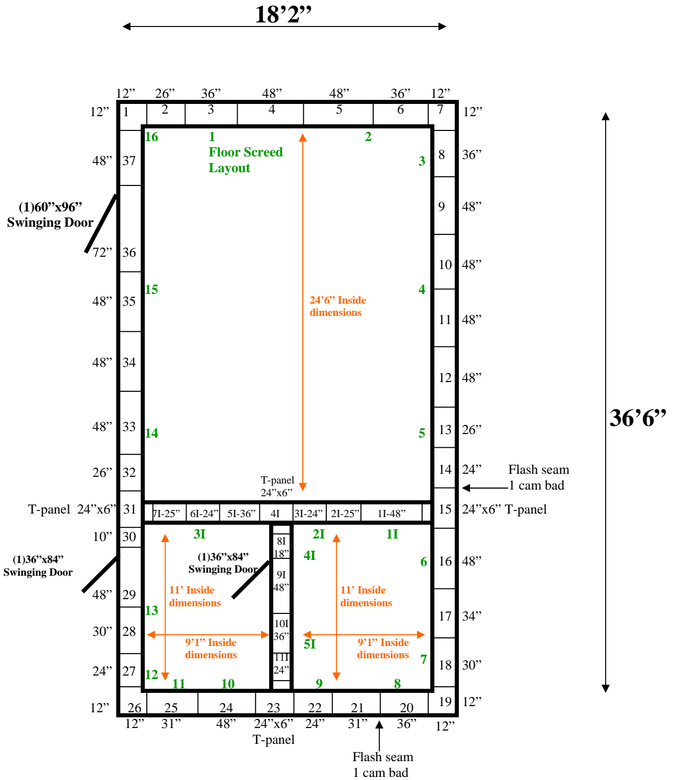
18'2" x 36'6" x 10'6" H Walk-In Combination Cooler / Freezer Wall Panels Diagram
